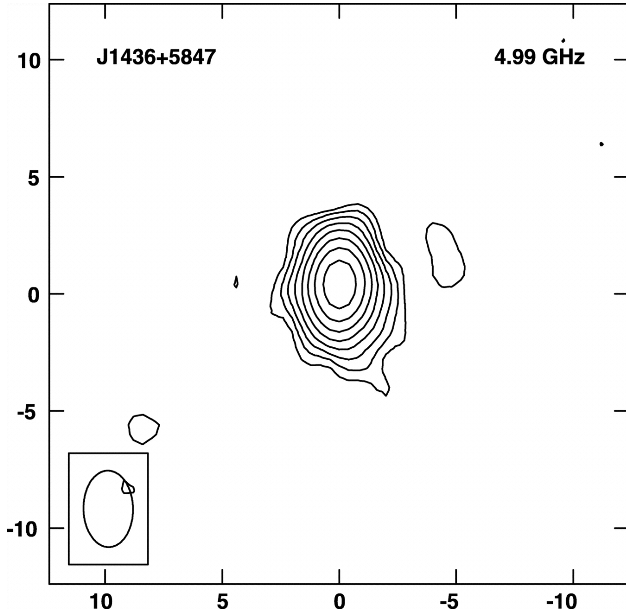
Fig. 1. from VLBA Imaging of Central Engines in RadioQuiet Quasars Ulvestad, Antonucci, & Barvainis 2005 ApJ 621 123 doi:10.1086/427426 https://dx.doi.org/10.1086/427426
