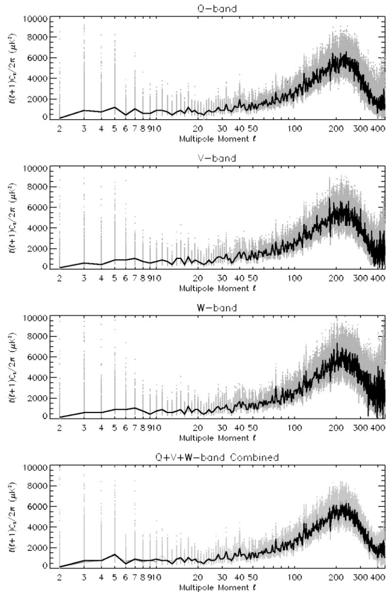
Fig. 2. from Bayesian Power Spectrum Analysis of the FirstYear Wilkinson Microwave Anisotropy Probe Data O'Dwyer et al. 2004 ApJL 617 L99 doi:10.1086/427386 https://dx.doi.org/10.1086/427386
