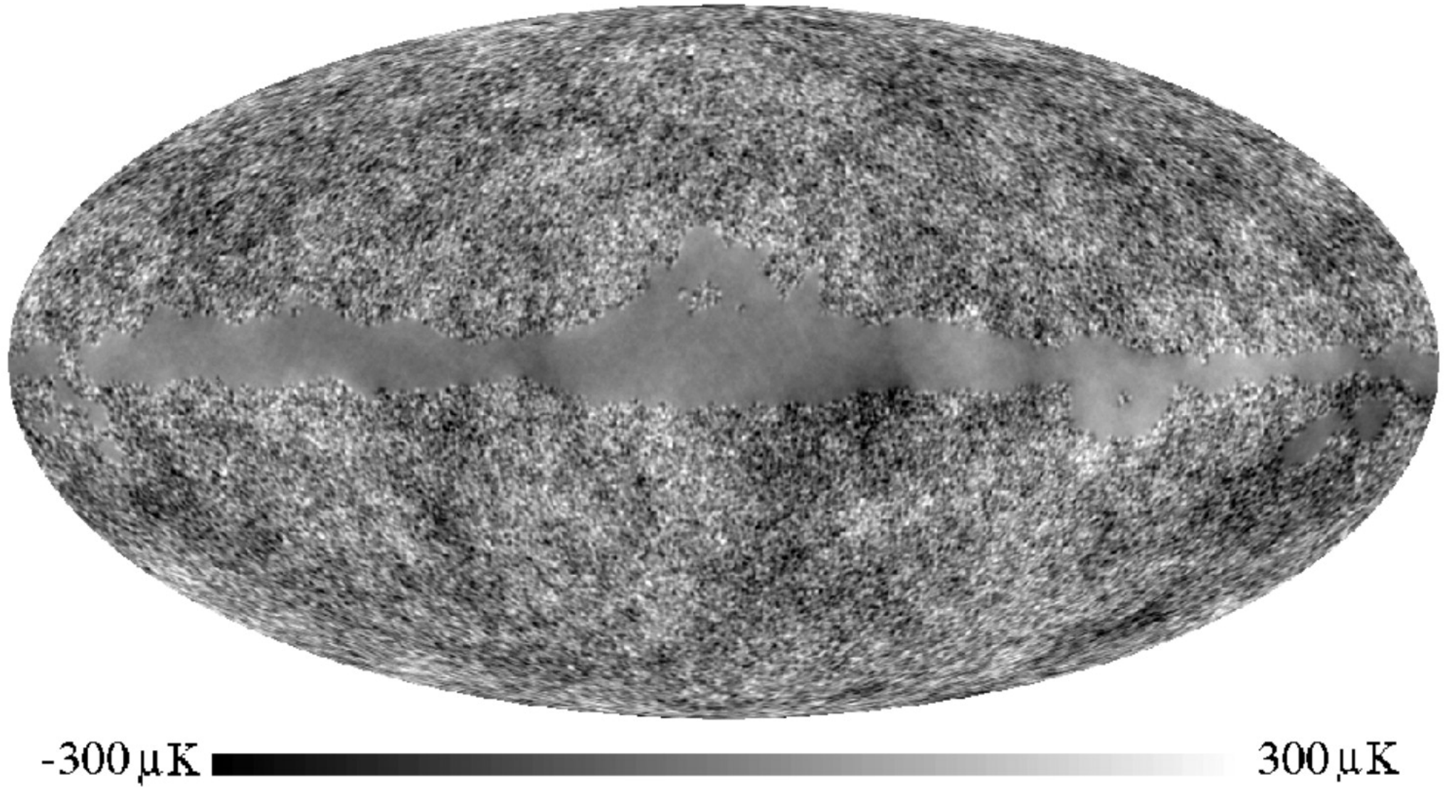
Fig. 1. from Bayesian Power Spectrum Analysis of the FirstYear Wilkinson Microwave Anisotropy Probe Data O'Dwyer et al. 2004 ApJL 617 L99 doi:10.1086/427386 https://dx.doi.org/10.1086/427386 © 2004. The American Astronomical Society. All rights reserved. Printed in U.S.A.
