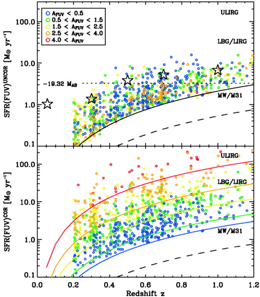
Fig. 4. from The GALEXVDS Measurement of the Evolution of the FarUltraviolet Luminosity Density and the Cosmic Star Formation Rate Schiminovich et al. 2005 ApJL 619 L47 doi:10.1086/427077 https://dx.doi.org/10.1086/427077
