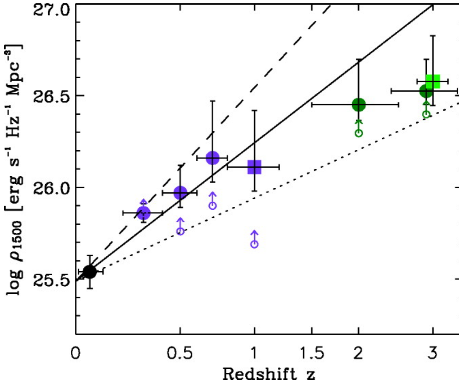
Fig. 1. from The GALEXVDS Measurement of the Evolution of the FarUltraviolet Luminosity Density and the Cosmic Star Formation Rate Schiminovich et al. 2005 ApJL 619 L47 doi:10.1086/427077 https://dx.doi.org/10.1086/427077 © 2005. The American Astronomical Society. All rights reserved. Printed in U.S.A.
