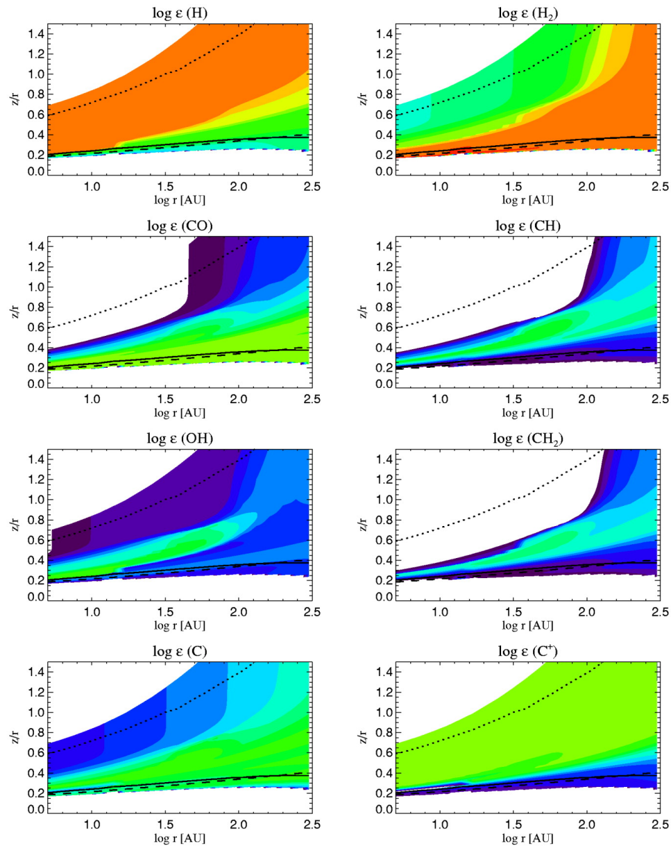
Fig. 7. from The Gas Temperature in the Surface Layers of Protoplanetary Disks Kamp & Dullemond 2004 ApJ 615 991 doi:10.1086/424703 https://dx.doi.org/10.1086/424703
