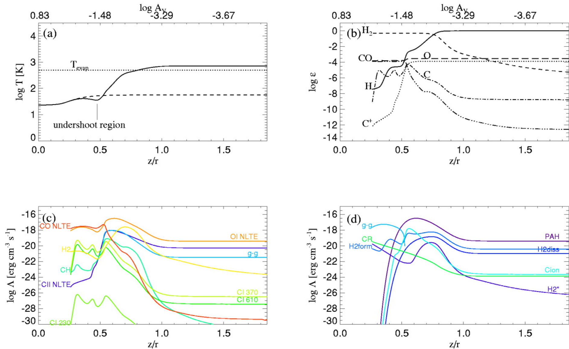
Fig. 6. from The Gas Temperature in the Surface Layers of Protoplanetary Disks Kamp & Dullemond 2004 ApJ 615 991 doi:10.1086/424703 https://dx.doi.org/10.1086/424703 © 2004. The American Astronomical Society. All rights reserved. Printed in U.S.A.
