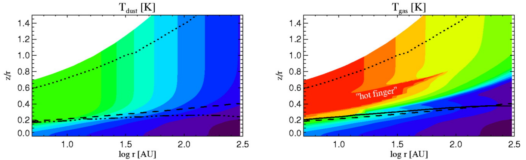
Fig. 2. from The Gas Temperature in the Surface Layers of Protoplanetary Disks Kamp & Dullemond 2004 ApJ 615 991 doi:10.1086/424703 https://dx.doi.org/10.1086/424703 © 2004. The American Astronomical Society. All rights reserved. Printed in U.S.A.
