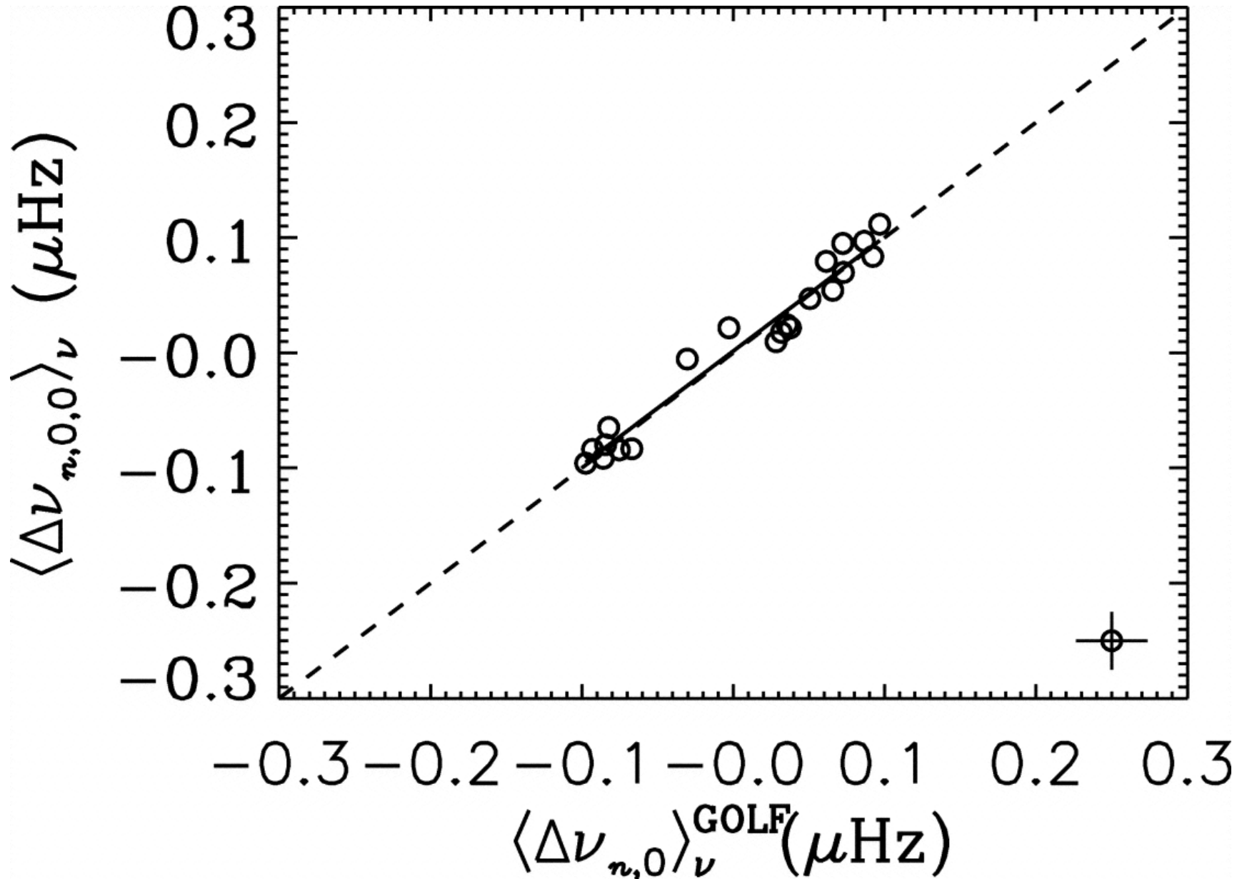
Fig. 2. from On the Spatial Dependence of LowDegree Solar pMode Frequency Shifts from FullDisk and ResolvedSun Observations JiménezReyes et al. 2004 ApJL 610 L65 doi:10.1086/423174 https://dx.doi.org/10.1086/423174 © 2004. The American Astronomical Society. All rights reserved. Printed in U.S.A.
