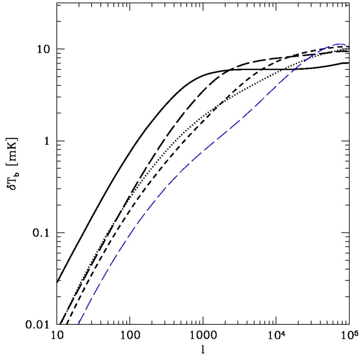
Fig. 8. from The Growth of H II Regions During Reionization Furlanetto, Zaldarriaga, & Hernquist 2004 ApJ 613 1 doi:10.1086/423025 https://dx.doi.org/10.1086/423025 © 2004. The American Astronomical Society. All rights reserved. Printed in U.S.A.
