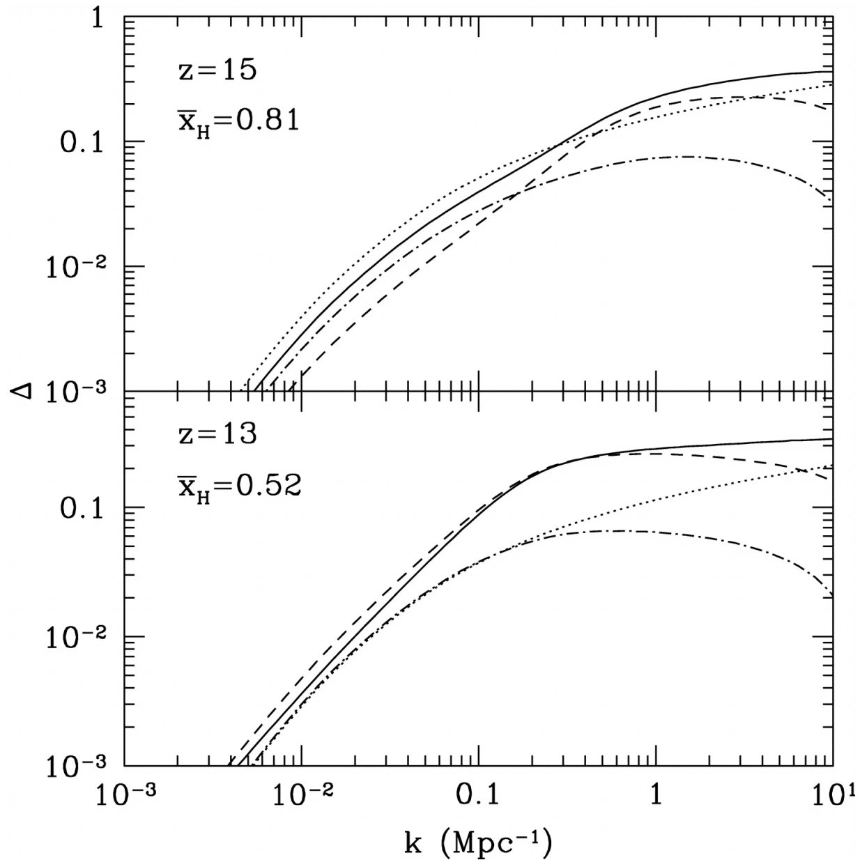
Fig. 6. from The Growth of H II Regions During Reionization Furlanetto, Zaldarriaga, & Hernquist 2004 ApJ 613 1 doi:10.1086/423025 https://dx.doi.org/10.1086/423025 © 2004. The American Astronomical Society. All rights reserved. Printed in U.S.A.
