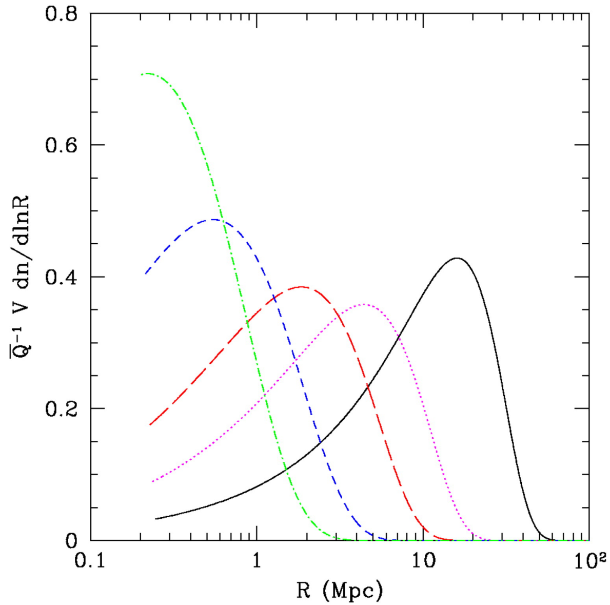
Fig. 2. from The Growth of H II Regions During Reionization Furlanetto, Zaldarriaga, & Hernquist 2004 ApJ 613 1 doi:10.1086/423025 https://dx.doi.org/10.1086/423025 © 2004. The American Astronomical Society. All rights reserved. Printed in U.S.A.
