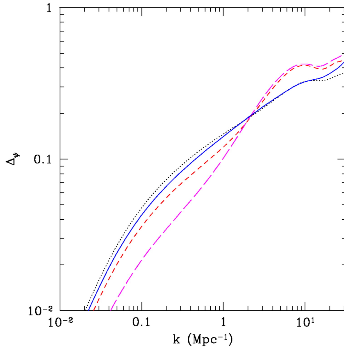
Fig. 11. from The Growth of H II Regions During Reionization Furlanetto, Zaldarriaga, & Hernquist 2004 ApJ 613 1 doi:10.1086/423025 https://dx.doi.org/10.1086/423025 © 2004. The American Astronomical Society. All rights reserved. Printed in U.S.A.
