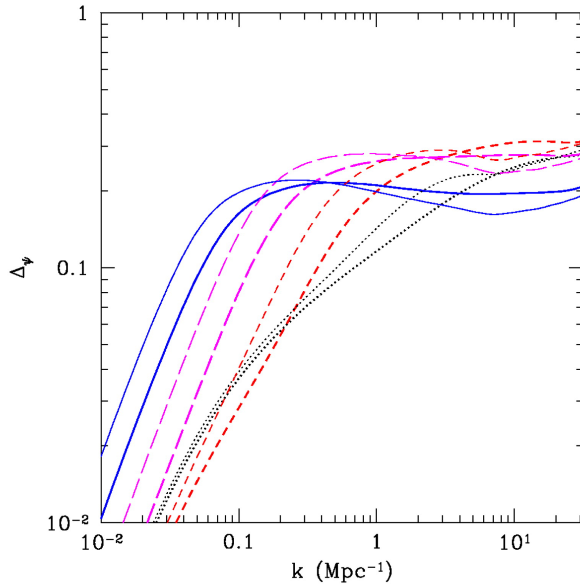
Fig. 10. from The Growth of H II Regions During Reionization Furlanetto, Zaldarriaga, & Hernquist 2004 ApJ 613 1 doi:10.1086/423025 https://dx.doi.org/10.1086/423025 © 2004. The American Astronomical Society. All rights reserved. Printed in U.S.A.
