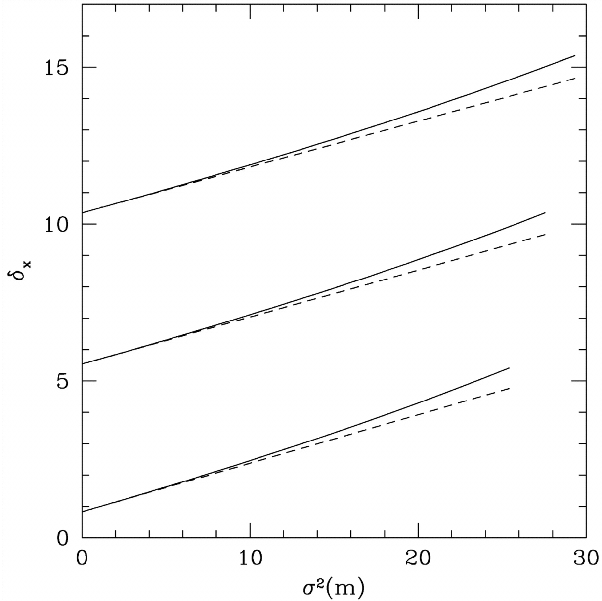
Fig. 1. from The Growth of H II Regions During Reionization Furlanetto, Zaldarriaga, & Hernquist 2004 ApJ 613 1 doi:10.1086/423025 https://dx.doi.org/10.1086/423025 © 2004. The American Astronomical Society. All rights reserved. Printed in U.S.A.
