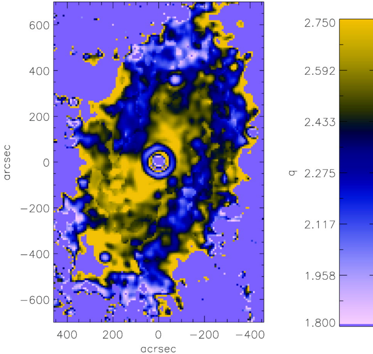
Fig. 6. from Spatially Resolved Ultraviolet, H, Infrared, and Radio Star Formation in M81 Gordon et al. 2004 ApJS 154 215 doi:10.1086/422714 https://dx.doi.org/10.1086/422714 © 2004. The American Astronomical Society. All rights reserved. Printed in U.S.A.
