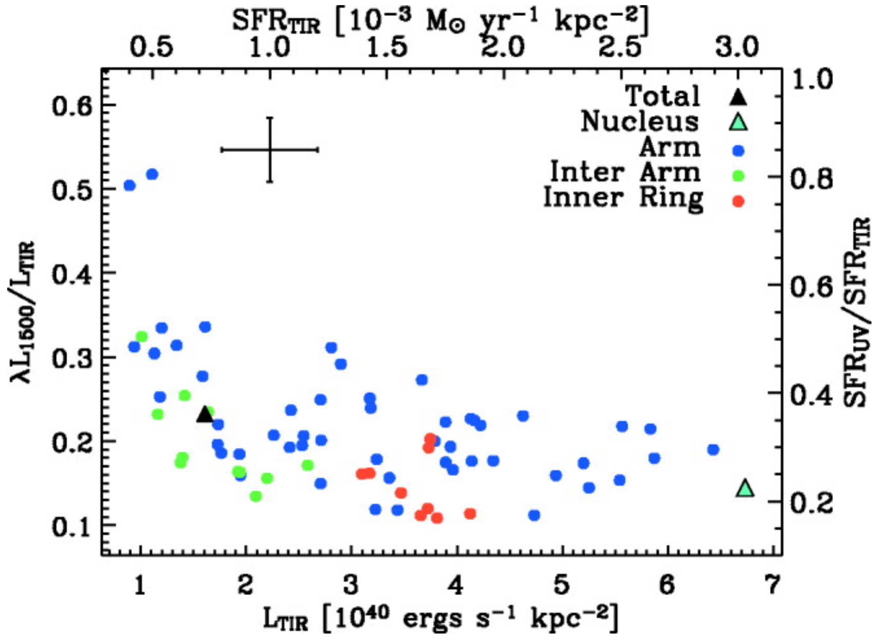
Fig. 4. from Spatially Resolved Ultraviolet, H, Infrared, and Radio Star Formation in M81 Gordon et al. 2004 ApJS 154 215 doi:10.1086/422714 https://dx.doi.org/10.1086/422714
