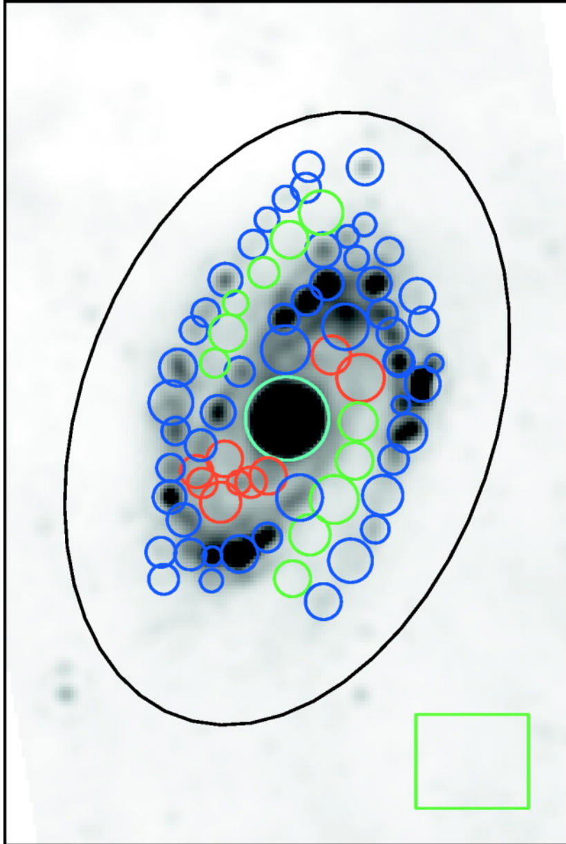
Fig. 3. from Spatially Resolved Ultraviolet, H, Infrared, and Radio Star Formation in M81 Gordon et al. 2004 ApJS 154 215 doi:10.1086/422714 https://dx.doi.org/10.1086/422714 © 2004. The American Astronomical Society. All rights reserved. Printed in U.S.A.
