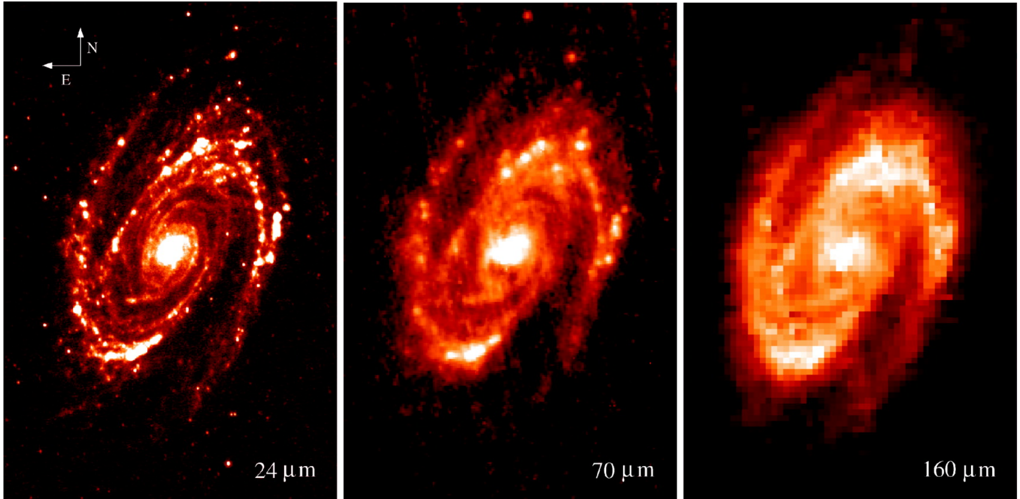
Fig. 1. from Spatially Resolved Ultraviolet, H, Infrared, and Radio Star Formation in M81 Gordon et al. 2004 ApJS 154 215 doi:10.1086/422714 https://dx.doi.org/10.1086/422714 © 2004. The American Astronomical Society. All rights reserved. Printed in U.S.A.
