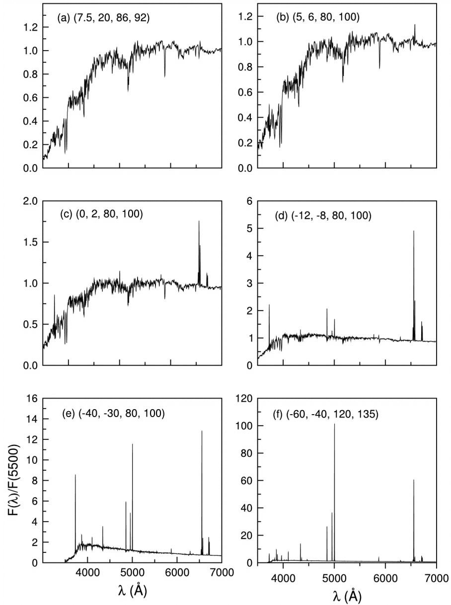
Fig. 9. from Distributions of Galaxy Spectral Types in the Sloan Digital Sky Survey Yip et al. 2004 AJ 128 585 doi:10.1086/422429 https://dx.doi.org/10.1086/422429 © 2004. The American Astronomical Society. All rights reserved. Printed in U.S.A.
