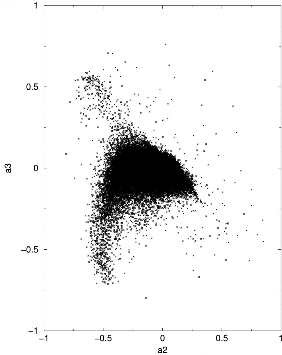
Fig. 7. from Distributions of Galaxy Spectral Types in the Sloan Digital Sky Survey Yip et al. 2004 AJ 128 585 doi:10.1086/422429 https://dx.doi.org/10.1086/422429 © 2004. The American Astronomical Society. All rights reserved. Printed in U.S.A.
