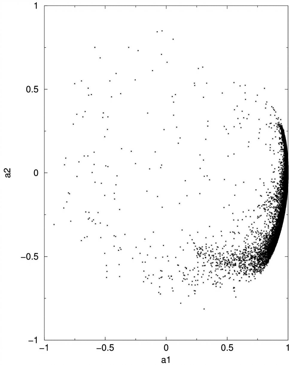
Fig. 6. from Distributions of Galaxy Spectral Types in the Sloan Digital Sky Survey Yip et al. 2004 AJ 128 585 doi:10.1086/422429 https://dx.doi.org/10.1086/422429 © 2004. The American Astronomical Society. All rights reserved. Printed in U.S.A.
