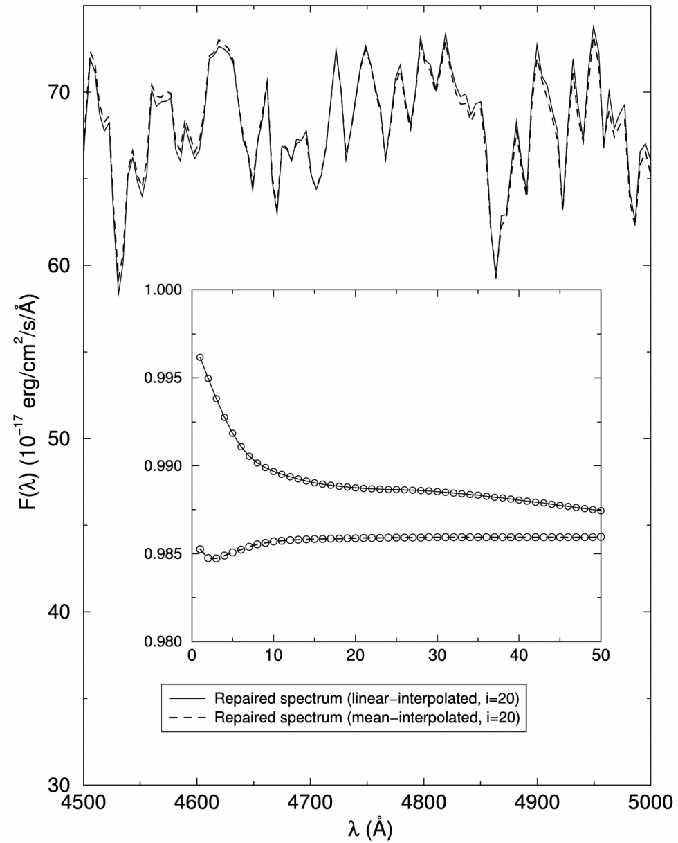
Fig. 3. from Distributions of Galaxy Spectral Types in the Sloan Digital Sky Survey Yip et al. 2004 AJ 128 585 doi:10.1086/422429 https://dx.doi.org/10.1086/422429 © 2004. The American Astronomical Society. All rights reserved. Printed in U.S.A.
