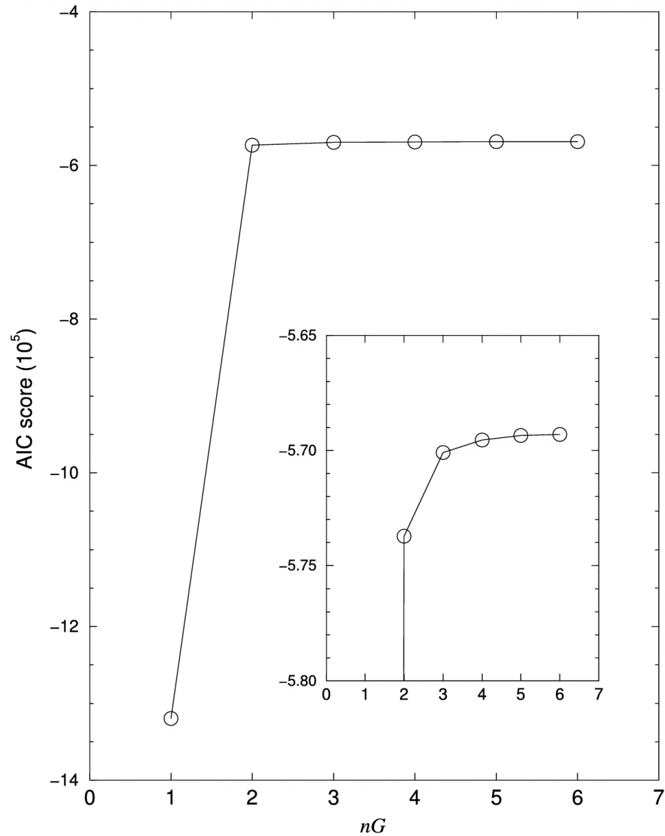
Fig. 19. from Distributions of Galaxy Spectral Types in the Sloan Digital Sky Survey Yip et al. 2004 AJ 128 585 doi:10.1086/422429 https://dx.doi.org/10.1086/422429 © 2004. The American Astronomical Society. All rights reserved. Printed in U.S.A.
