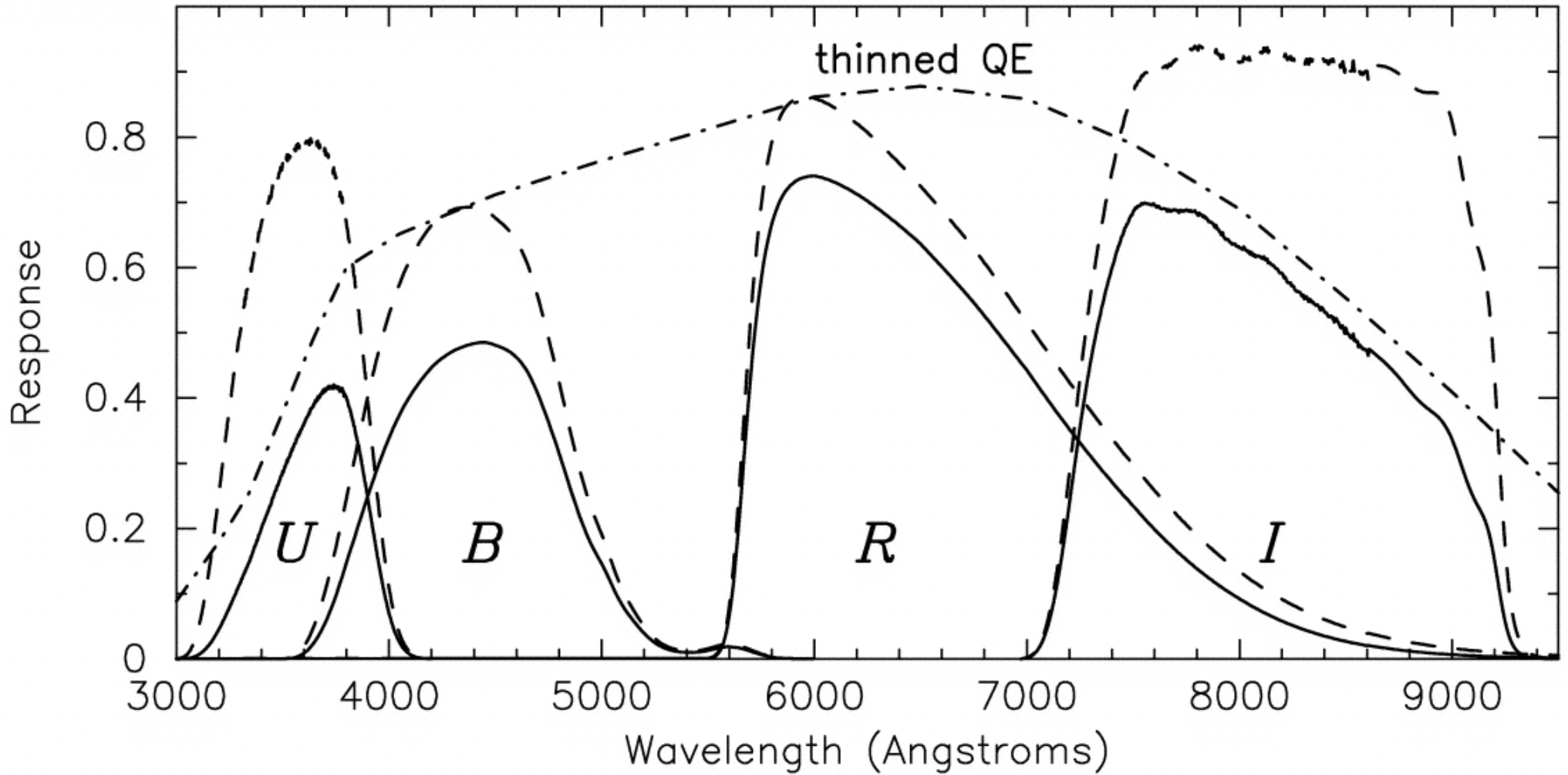
Fig. 1. from Quasars as Absorption Probes of the J0053+1234 Region McIntosh, Impey, & Petry 2004 AJ 128 544 doi:10.1086/422347 https://dx.doi.org/10.1086/422347 © 2004. The American Astronomical Society. All rights reserved. Printed in U.S.A.
