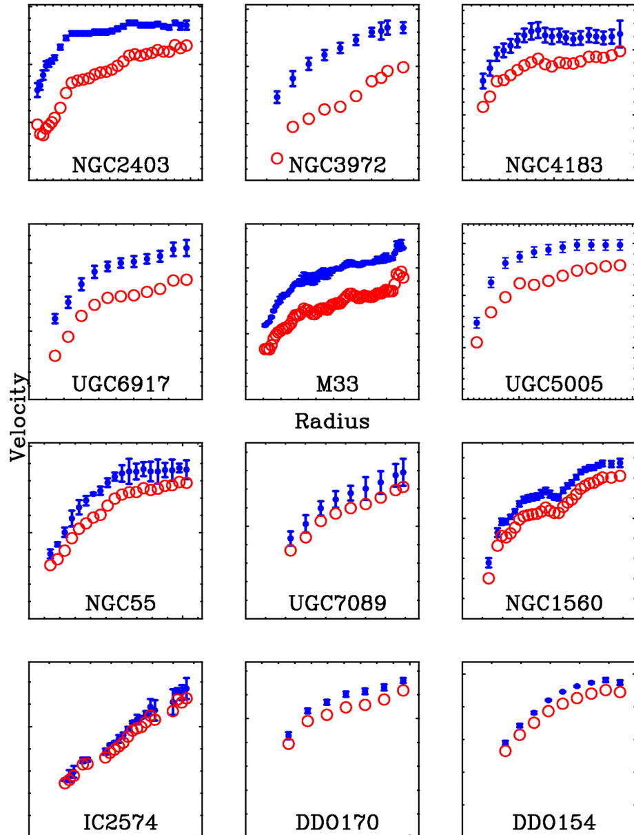
Fig. 9. from The Mass Discrepancy–Acceleration Relation: Disk Mass and the Dark Matter Distribution McGaugh 2004 ApJ 609 652 doi:10.1086/421338 https://dx.doi.org/10.1086/421338
