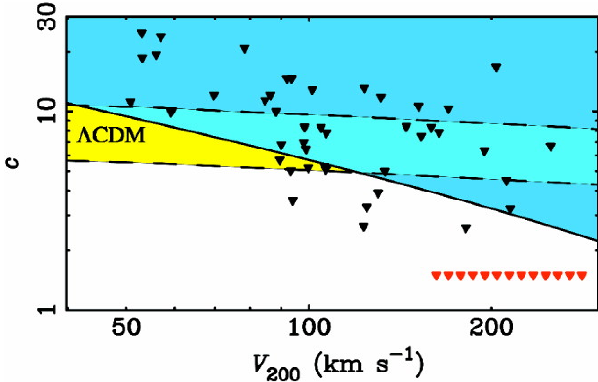
Fig. 8. from The Mass Discrepancy–Acceleration Relation: Disk Mass and the Dark Matter Distribution McGaugh 2004 ApJ 609 652 doi:10.1086/421338 https://dx.doi.org/10.1086/421338 © 2004. The American Astronomical Society. All rights reserved. Printed in U.S.A.
