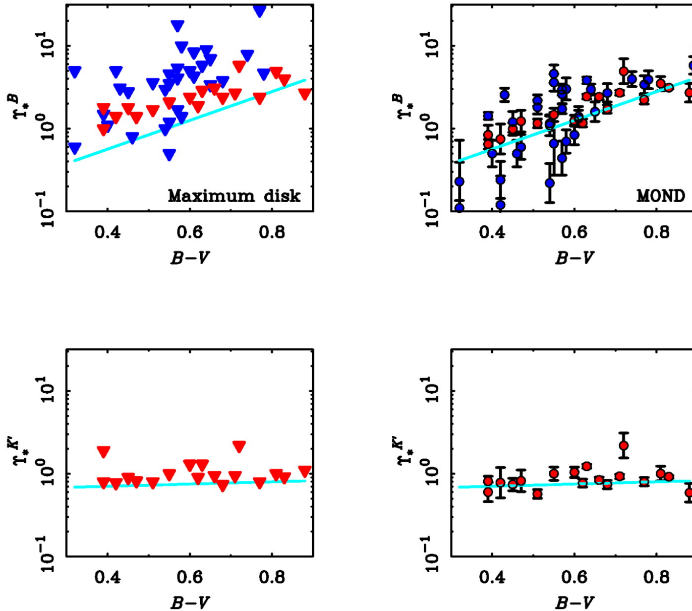
Fig. 7. from The Mass Discrepancy–Acceleration Relation: Disk Mass and the Dark Matter Distribution McGaugh 2004 ApJ 609 652 doi:10.1086/421338 https://dx.doi.org/10.1086/421338 © 2004. The American Astronomical Society. All rights reserved. Printed in U.S.A.
