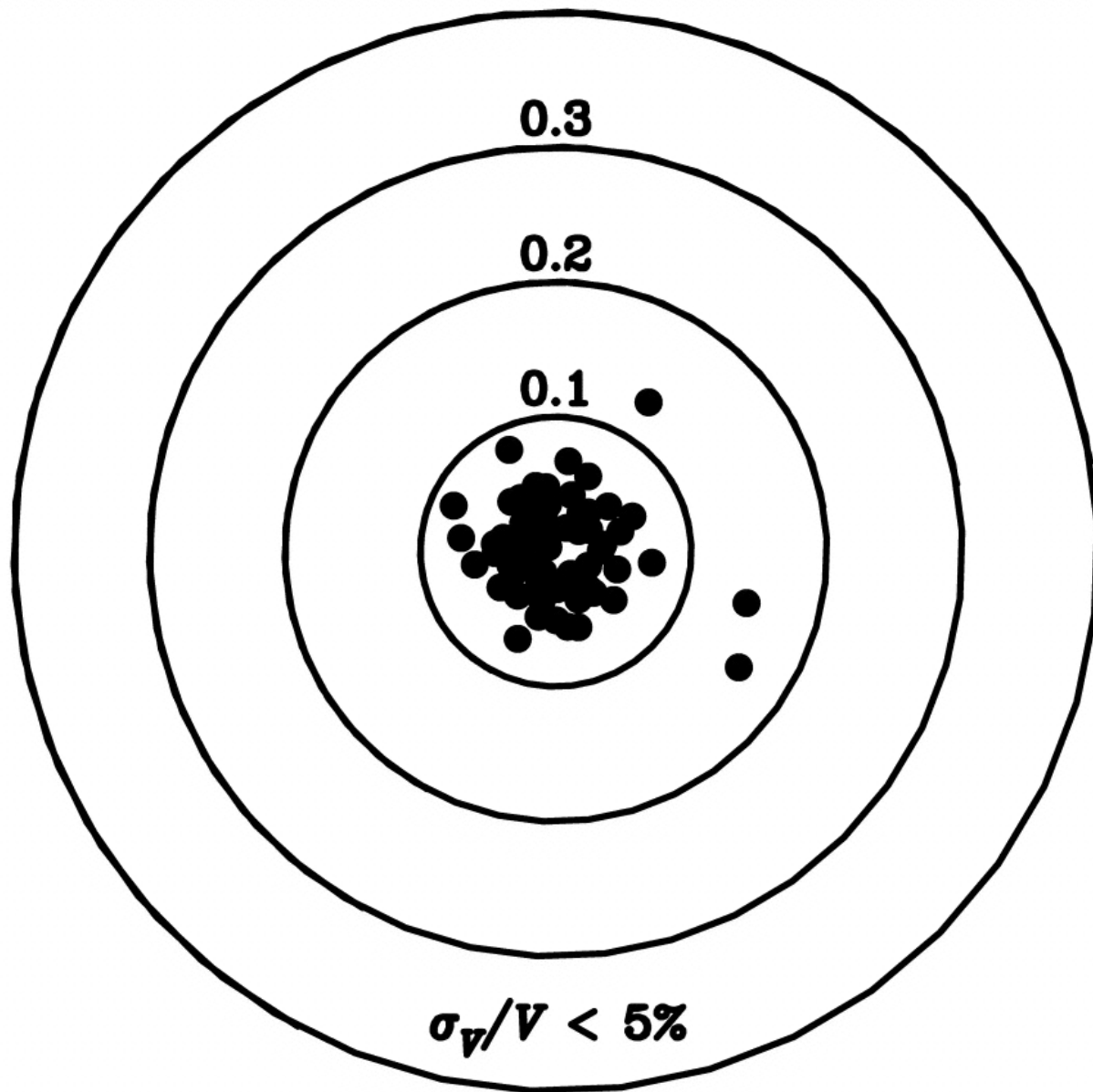
Fig. 2. from The Mass Discrepancy–Acceleration Relation: Disk Mass and the Dark Matter Distribution McGaugh 2004 ApJ 609 652 doi:10.1086/421338 https://dx.doi.org/10.1086/421338 © 2004. The American Astronomical Society. All rights reserved. Printed in U.S.A.
