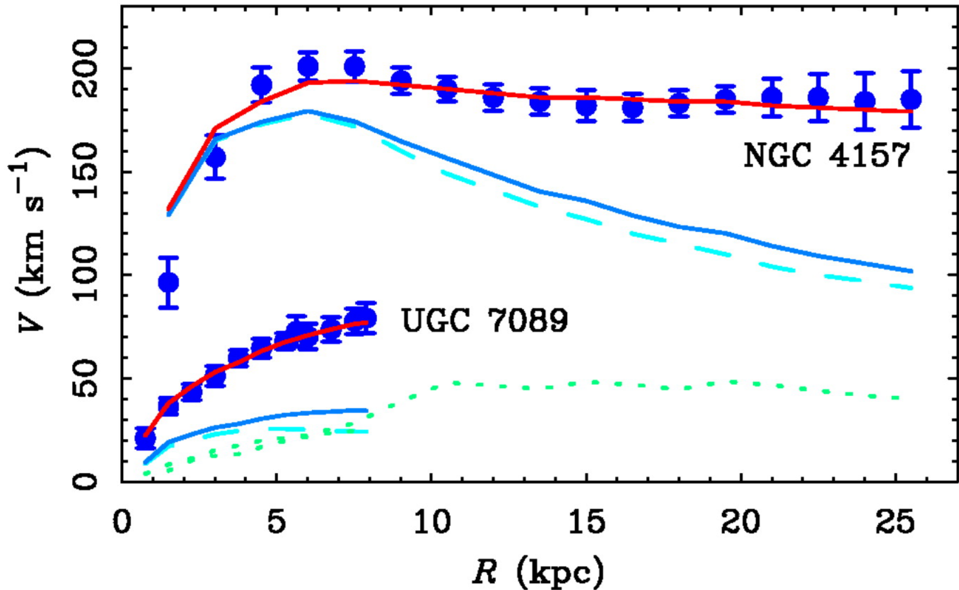
Fig. 1. from The Mass Discrepancy–Acceleration Relation: Disk Mass and the Dark Matter Distribution McGaugh 2004 ApJ 609 652 doi:10.1086/421338 https://dx.doi.org/10.1086/421338 © 2004. The American Astronomical Society. All rights reserved. Printed in U.S.A.
