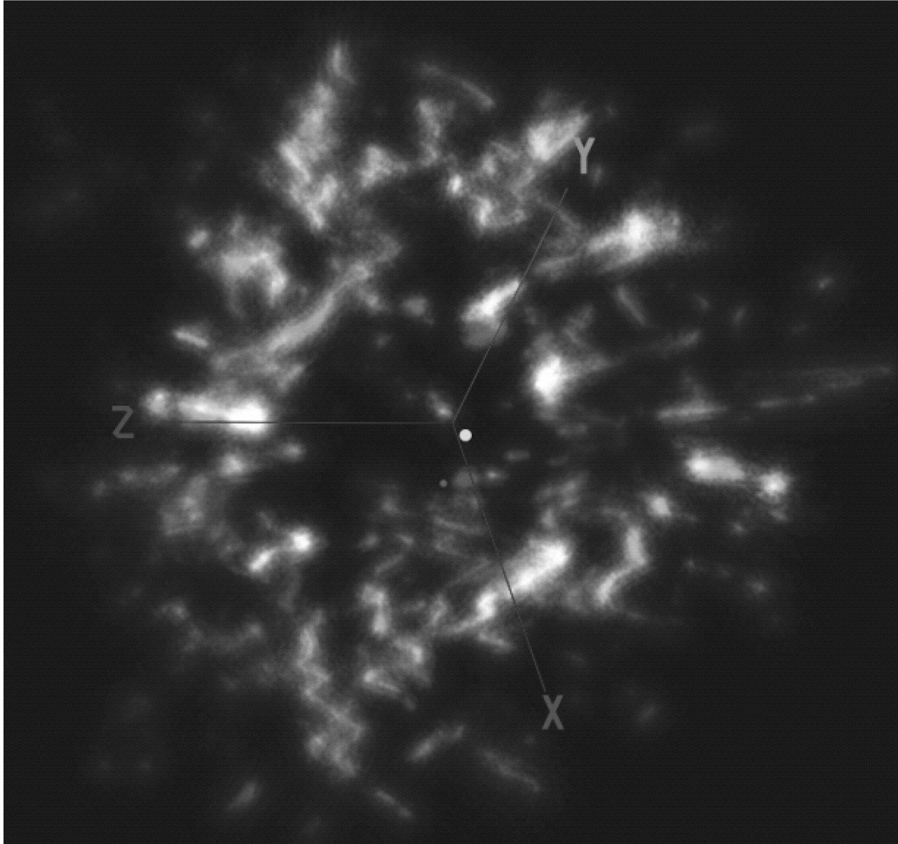
Fig. 12. from Spectroscopy and ThreeDimensional Imaging of the Crab Nebula adež, Carramiñana, & Vidrih 2004 ApJ 609 797 doi:10.1086/421234 https://dx.doi.org/10.1086/421234 © 2004. The American Astronomical Society. All rights reserved. Printed in U.S.A.
