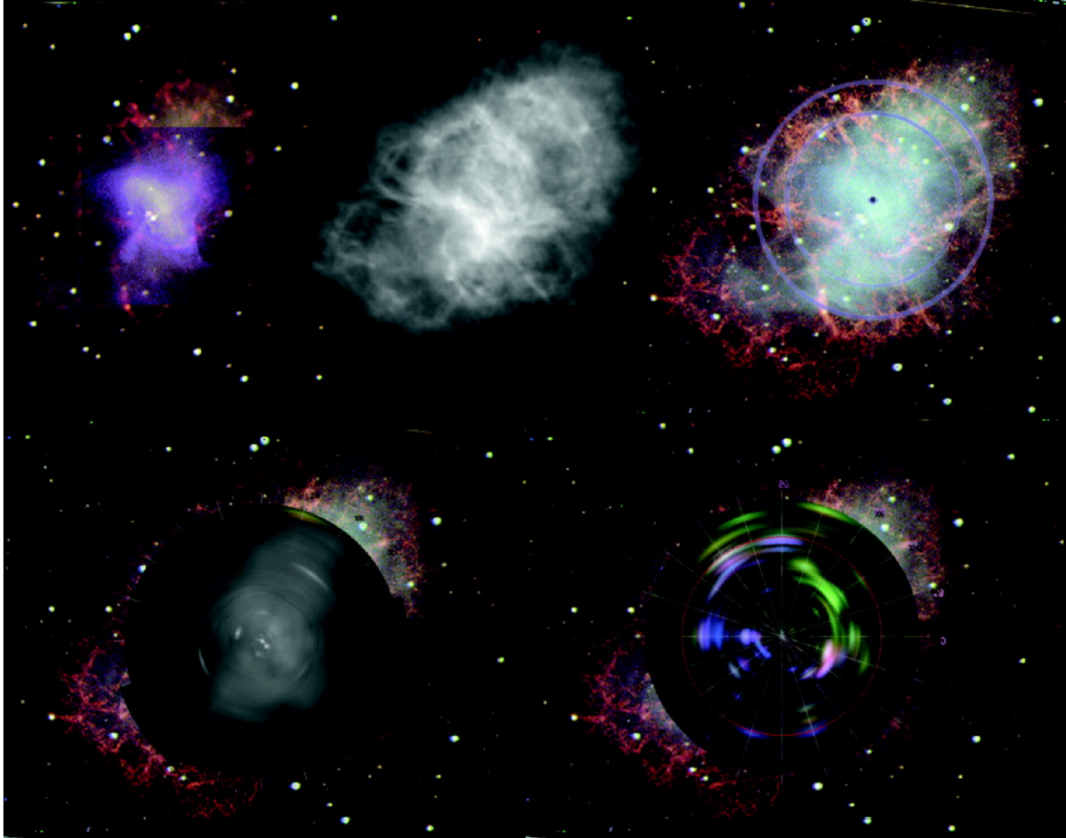
Fig. 11. from Spectroscopy and ThreeDimensional Imaging of the Crab Nebula adež, Carramiñana, & Vidrih 2004 ApJ 609 797 doi:10.1086/421234 https://dx.doi.org/10.1086/421234 © 2004. The American Astronomical Society. All rights reserved. Printed in U.S.A.
