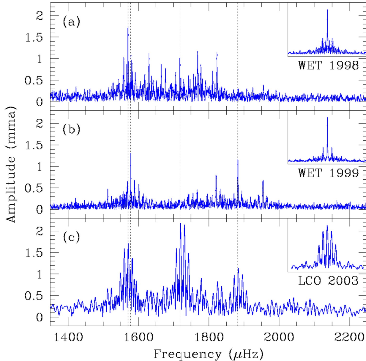
Fig. 1. from Testing White Dwarf Crystallization Theory with Asteroseismology of the Massive Pulsating DA Star BPM 37093 Metcalfe, Montgomery, & Kanaan 2004 ApJL 605 L133 doi:10.1086/420884 https://dx.doi.org/10.1086/420884
