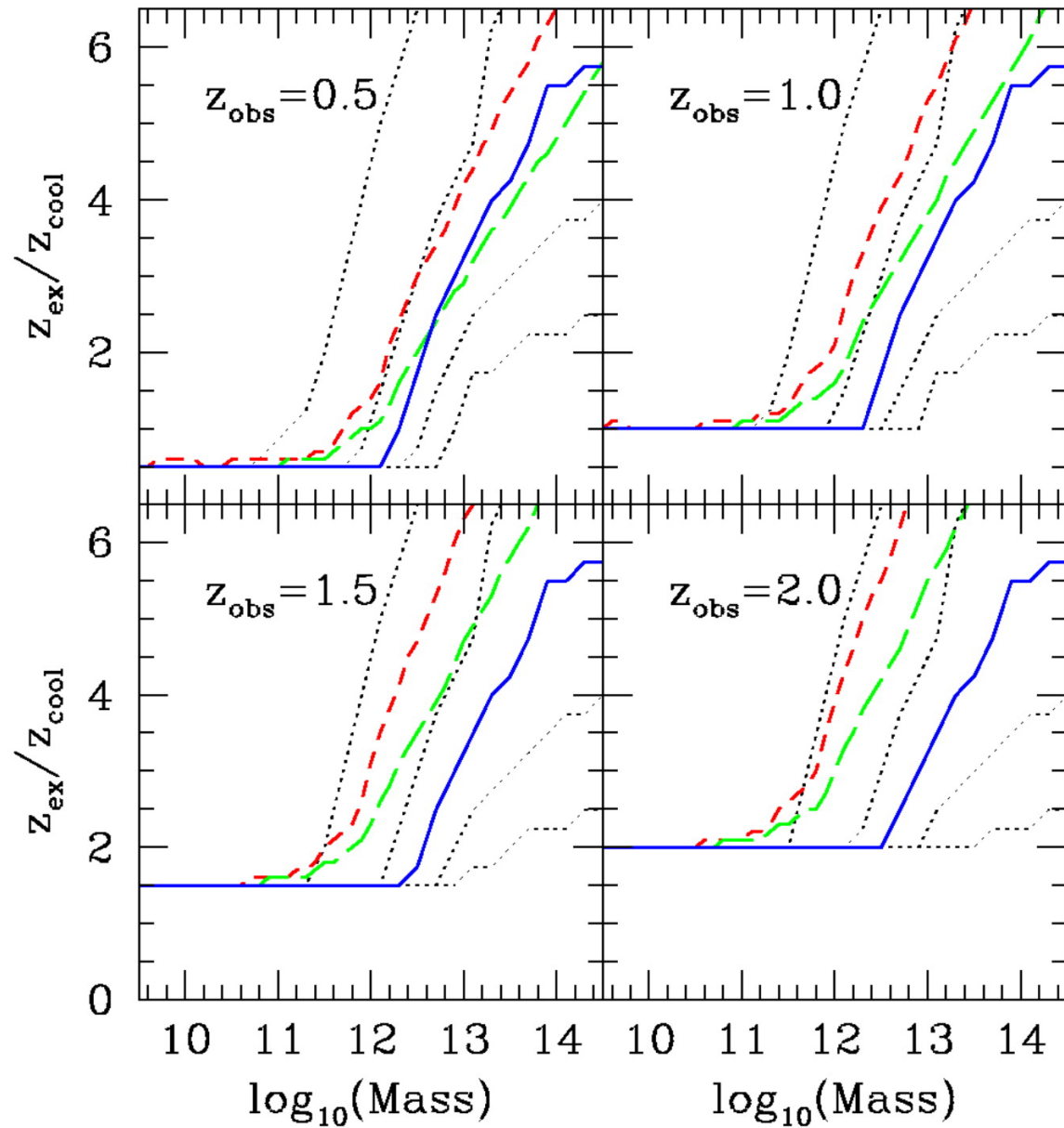
Fig. 9. from Quasar Feedback: The Missing Link in Structure Formation Scannapieco & Oh 2004 ApJ 608 62 doi:10.1086/386542 https://dx.doi.org/10.1086/386542 © 2004. The American Astronomical Society. All rights reserved. Printed in U.S.A.
