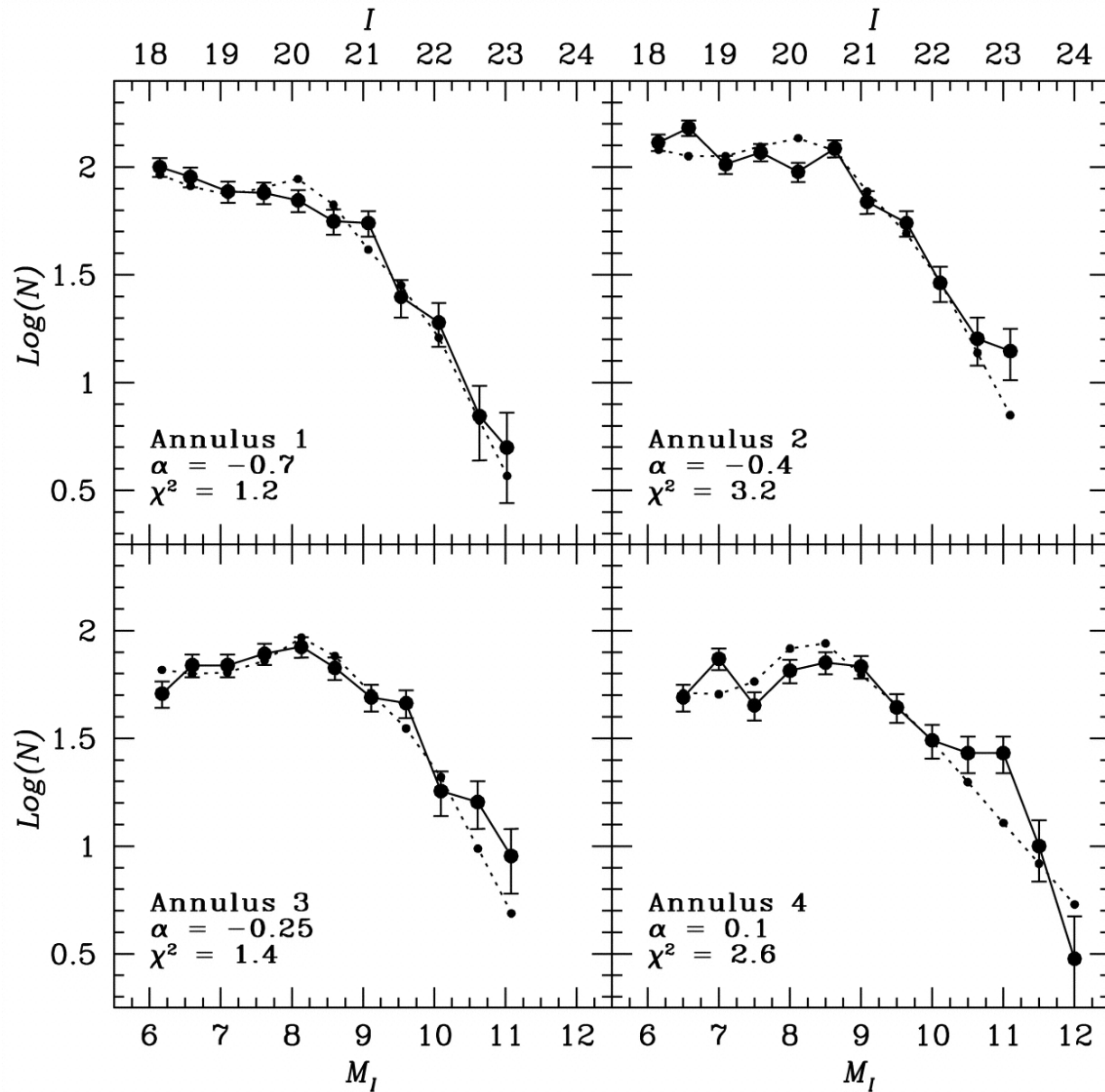
Fig. 9. from Hubble Space Telescope Observations of the Main Sequence of M4 Richer et al. 2004 AJ 127 2771 doi:10.1086/383543 https://dx.doi.org/10.1086/383543 © 2004. The American Astronomical Society. All rights reserved. Printed in U.S.A.
