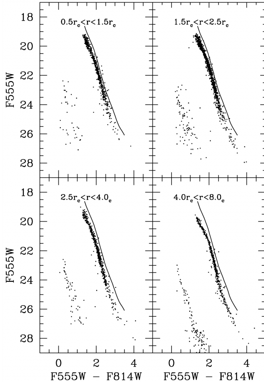
Fig. 5. from Hubble Space Telescope Observations of the Main Sequence of M4 Richer et al. 2004 AJ 127 2771 doi:10.1086/383543 https://dx.doi.org/10.1086/383543 © 2004. The American Astronomical Society. All rights reserved. Printed in U.S.A.
