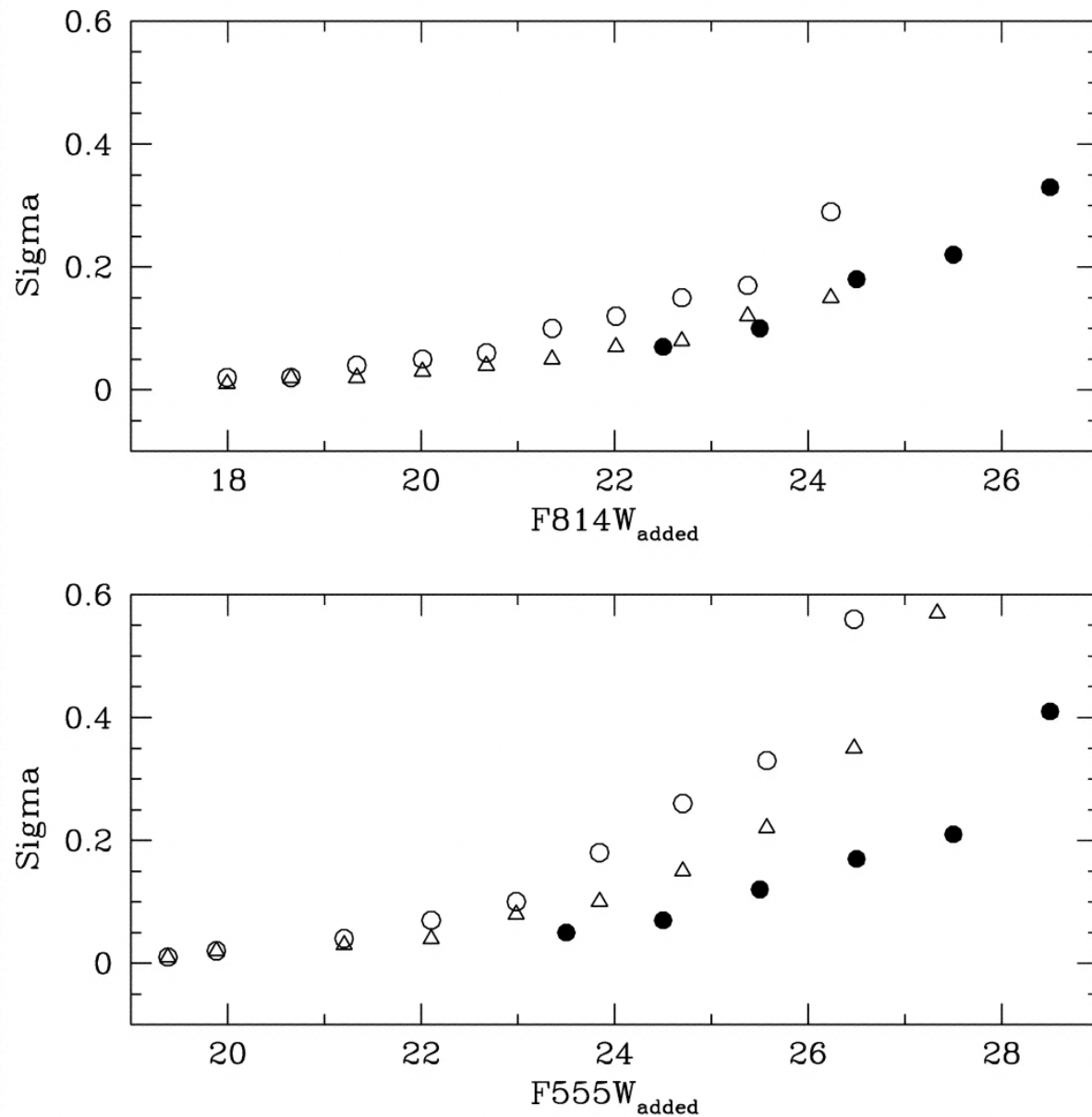
Fig. 4. from Hubble Space Telescope Observations of the Main Sequence of M4 Richer et al. 2004 AJ 127 2771 doi:10.1086/383543 https://dx.doi.org/10.1086/383543 © 2004. The American Astronomical Society. All rights reserved. Printed in U.S.A.
