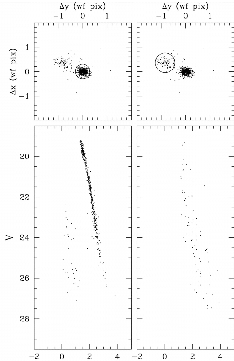
Fig. 3. from Hubble Space Telescope Observations of the Main Sequence of M4 Richer et al. 2004 AJ 127 2771 doi:10.1086/383543 https://dx.doi.org/10.1086/383543 © 2004. The American Astronomical Society. All rights reserved. Printed in U.S.A.
