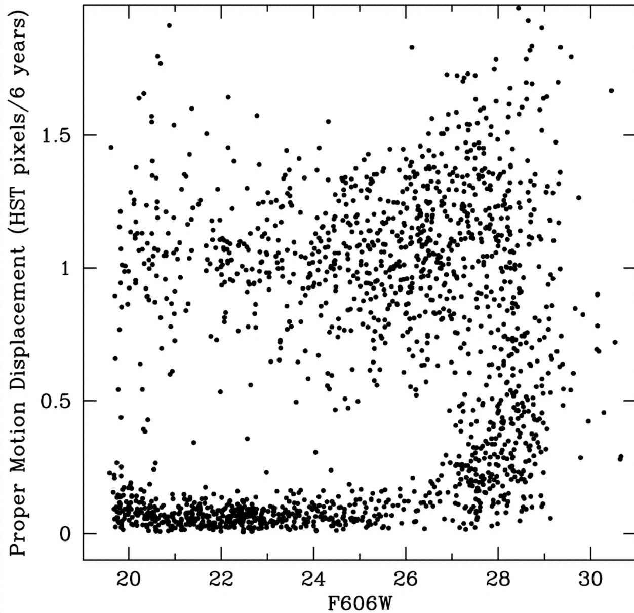
Fig. 2. from Hubble Space Telescope Observations of the Main Sequence of M4 Richer et al. 2004 AJ 127 2771 doi:10.1086/383543 https://dx.doi.org/10.1086/383543 © 2004. The American Astronomical Society. All rights reserved. Printed in U.S.A.
