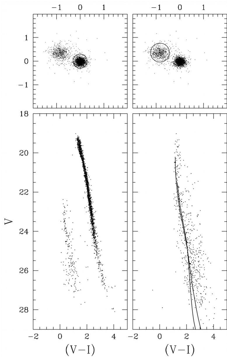
Fig. 14. from Hubble Space Telescope Observations of the Main Sequence of M4 Richer et al. 2004 AJ 127 2771 doi:10.1086/383543 https://dx.doi.org/10.1086/383543 © 2004. The American Astronomical Society. All rights reserved. Printed in U.S.A.
