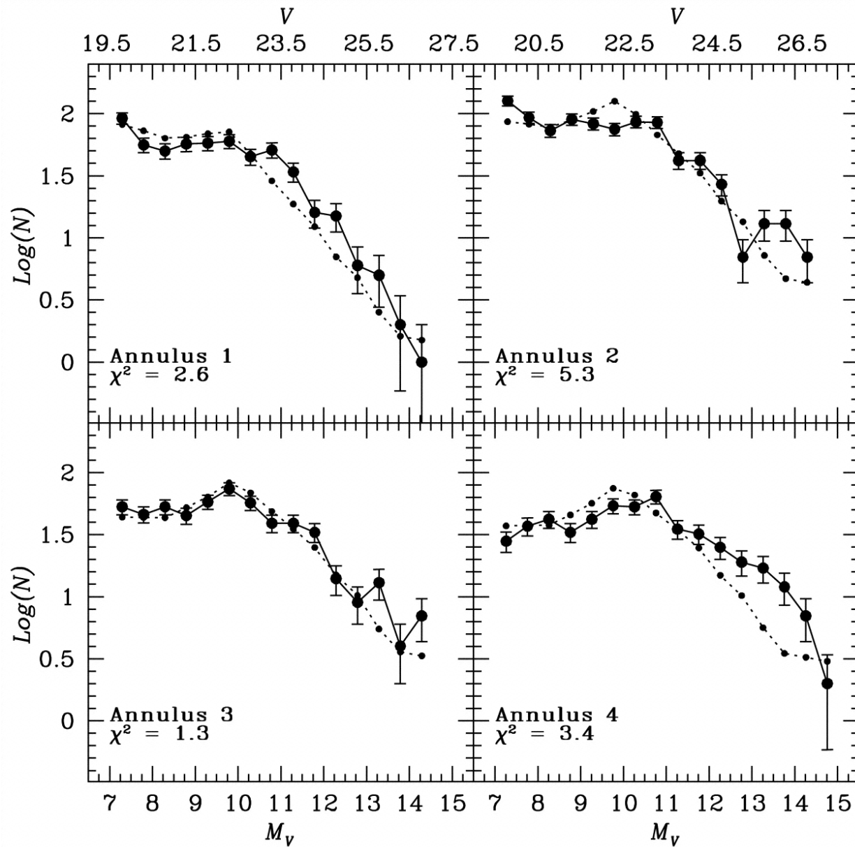
Fig. 12. from Hubble Space Telescope Observations of the Main Sequence of M4 Richer et al. 2004 AJ 127 2771 doi:10.1086/383543 https://dx.doi.org/10.1086/383543 © 2004. The American Astronomical Society. All rights reserved. Printed in U.S.A.
