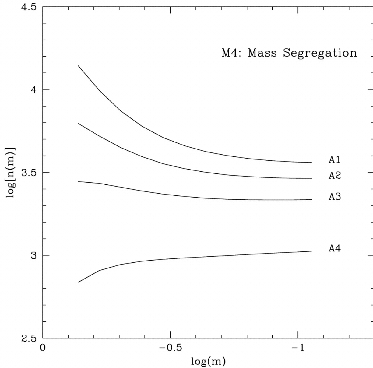
Fig. 11. from Hubble Space Telescope Observations of the Main Sequence of M4 Richer et al. 2004 AJ 127 2771 doi:10.1086/383543 https://dx.doi.org/10.1086/383543 © 2004. The American Astronomical Society. All rights reserved. Printed in U.S.A.
