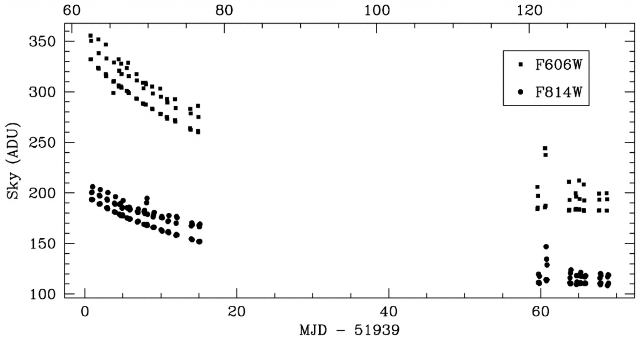
Fig. 1. from Hubble Space Telescope Observations of the Main Sequence of M4 Richer et al. 2004 AJ 127 2771 doi:10.1086/383543 https://dx.doi.org/10.1086/383543 © 2004. The American Astronomical Society. All rights reserved. Printed in U.S.A.
