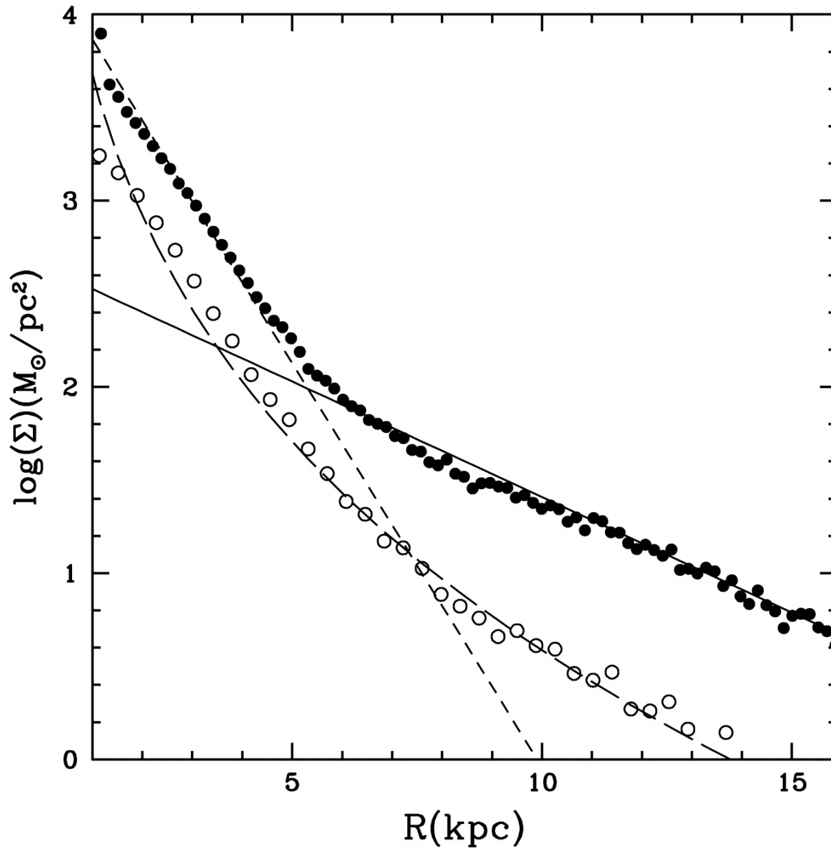
Fig. 2. from The Formation of a Realistic Disk Galaxy in dominated Cosmologies Governato et al. 2004 ApJ 607 688 doi:10.1086/383516 https://dx.doi.org/10.1086/383516 © 2004. The American Astronomical Society. All rights reserved. Printed in U.S.A.
