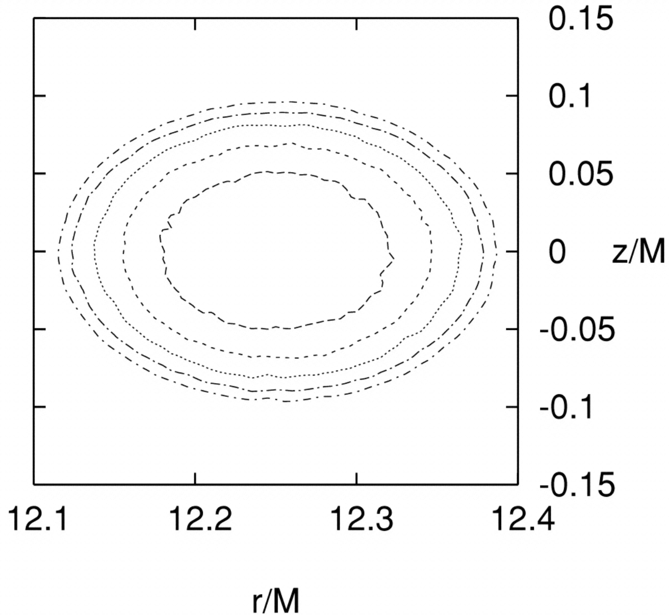
Fig. 1. from Resonance in Forced Oscillations of an Accretion Disk and Kilohertz Quasiperiodic Oscillations Lee, Abramowicz, & Kluniak 2004 ApJL 603 L93 doi:10.1086/383245 https://dx.doi.org/10.1086/383245 © 2004. The American Astronomical Society. All rights reserved. Printed in U.S.A.
