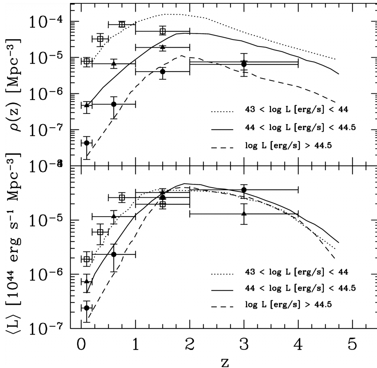
Fig. 8. from XRay Evolution of Active Galactic Nuclei and Hierarchical Galaxy Formation Menci et al. 2004 ApJ 606 58 doi:10.1086/382780 https://dx.doi.org/10.1086/382780 © 2004. The American Astronomical Society. All rights reserved. Printed in U.S.A.
