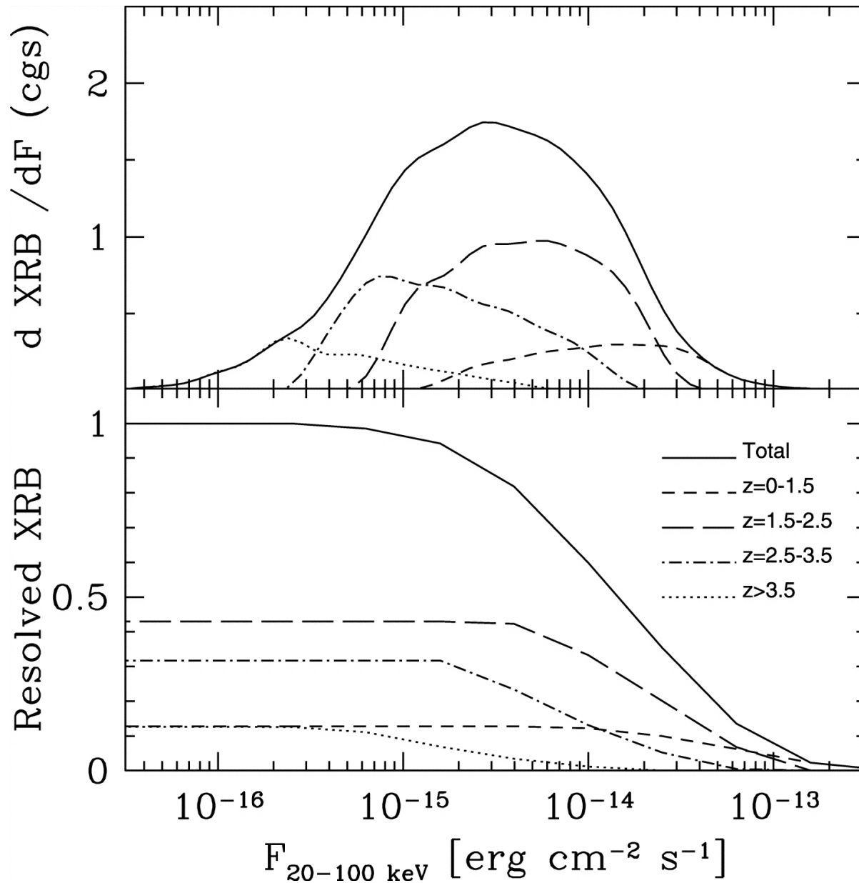
Fig. 6. from XRay Evolution of Active Galactic Nuclei and Hierarchical Galaxy Formation Menci et al. 2004 ApJ 606 58 doi:10.1086/382780 https://dx.doi.org/10.1086/382780 © 2004. The American Astronomical Society. All rights reserved. Printed in U.S.A.
