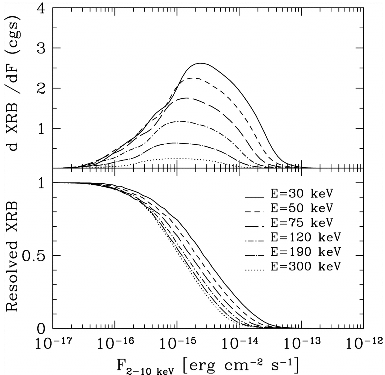
Fig. 5. from XRay Evolution of Active Galactic Nuclei and Hierarchical Galaxy Formation Menci et al. 2004 ApJ 606 58 doi:10.1086/382780 https://dx.doi.org/10.1086/382780 © 2004. The American Astronomical Society. All rights reserved. Printed in U.S.A.
