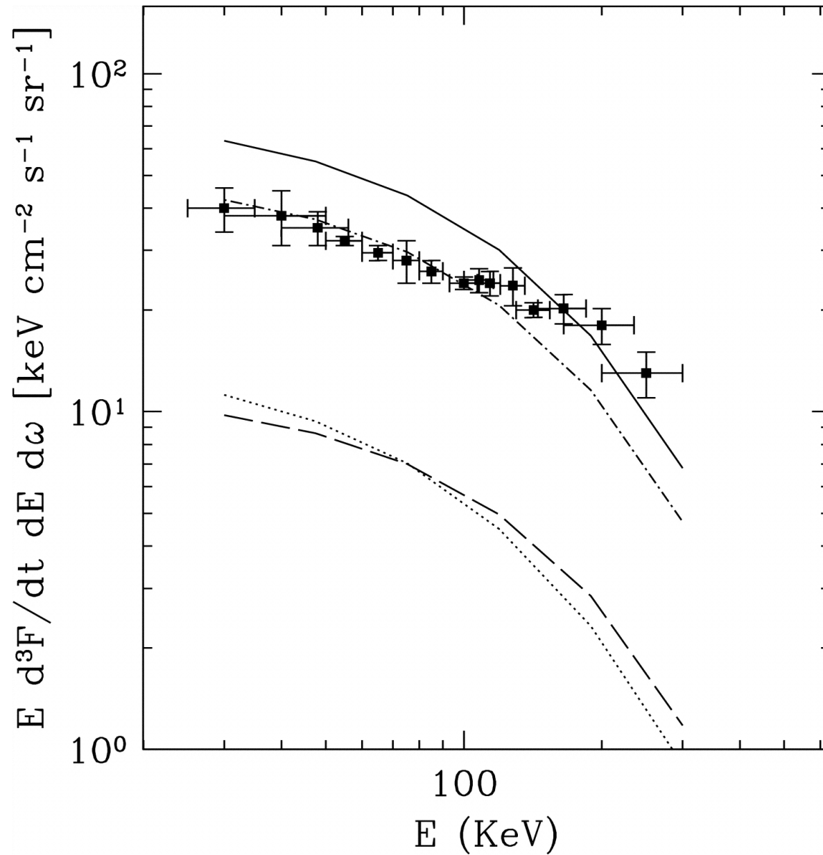
Fig. 4. from XRay Evolution of Active Galactic Nuclei and Hierarchical Galaxy Formation Menci et al. 2004 ApJ 606 58 doi:10.1086/382780 https://dx.doi.org/10.1086/382780 © 2004. The American Astronomical Society. All rights reserved. Printed in U.S.A.
