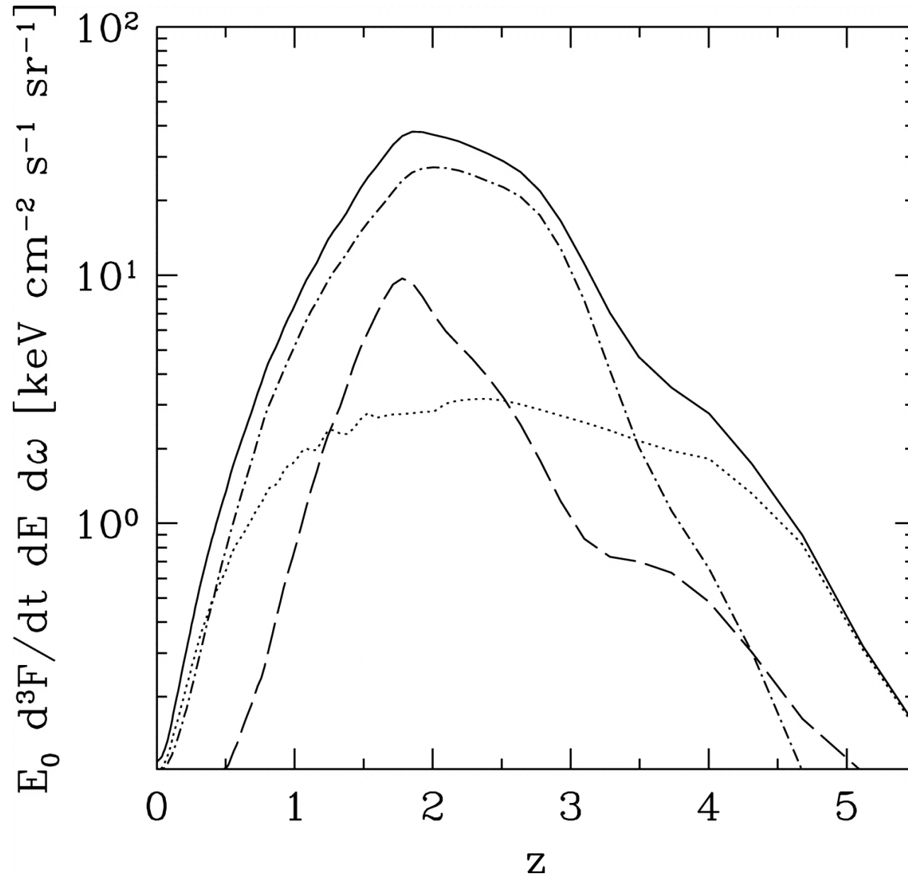
Fig. 3. from XRay Evolution of Active Galactic Nuclei and Hierarchical Galaxy Formation Menci et al. 2004 ApJ 606 58 doi:10.1086/382780 https://dx.doi.org/10.1086/382780 © 2004. The American Astronomical Society. All rights reserved. Printed in U.S.A.
